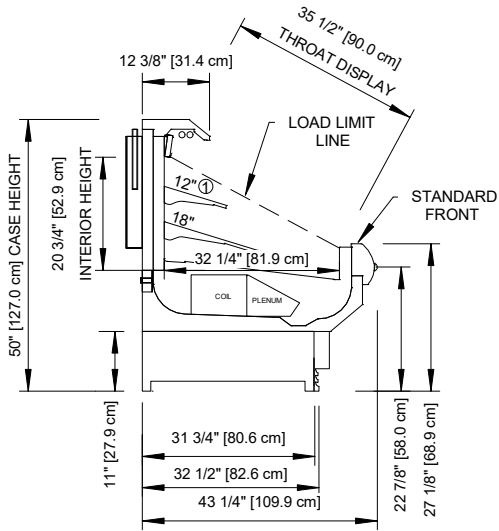
11" BASE FRAME
