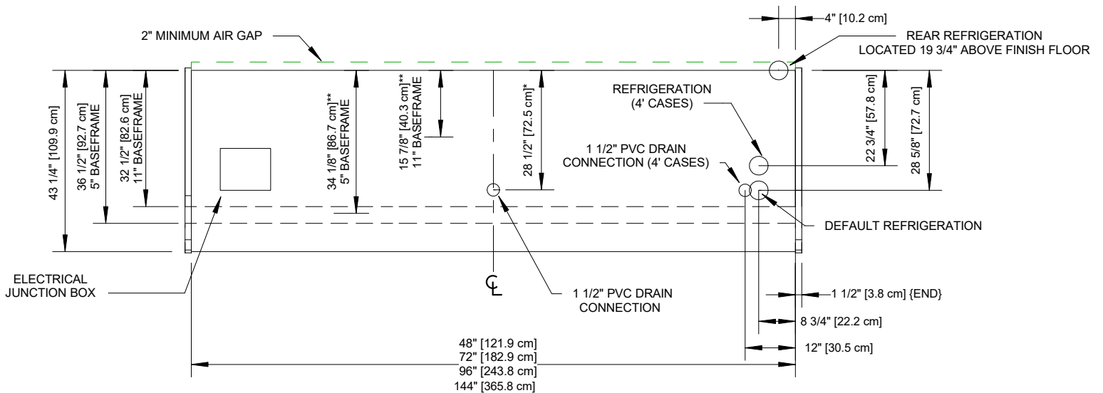
11" BASEFRAME
