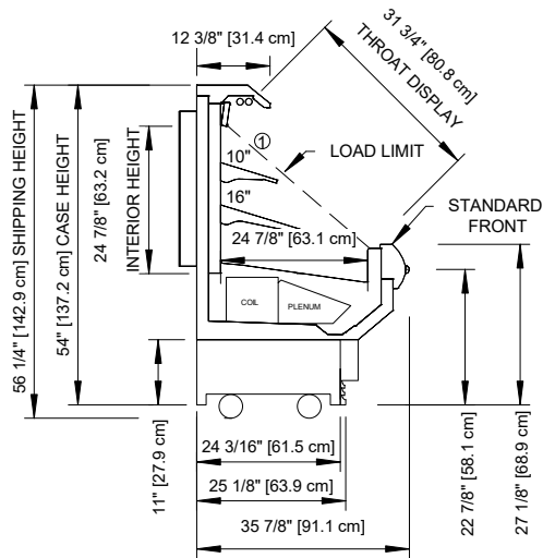
11" BASE FRAME
