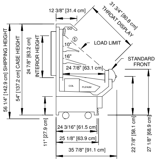
11" BASE FRAME
