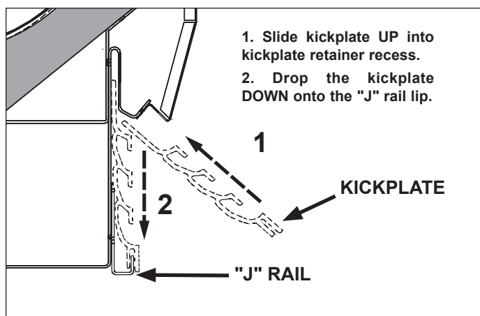
Fig. 3 Kickplate installation
