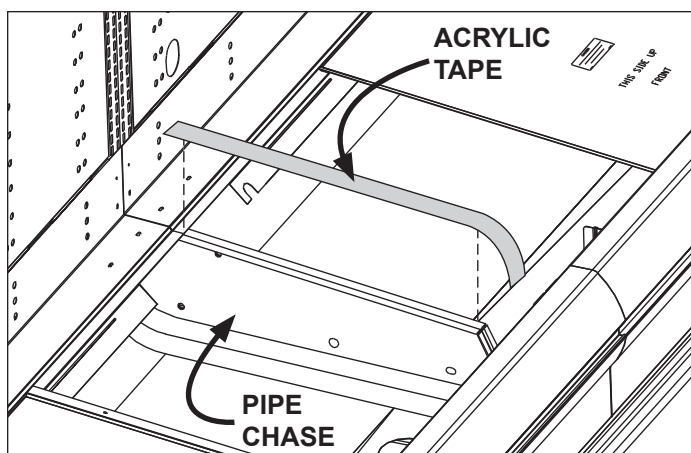
Fig. 2 Sealing the pipe chase
