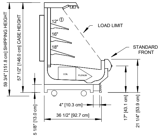
5" BASEFRAME
