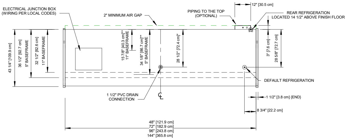
11" BASEFRAME
