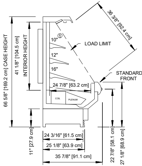
11" BASEFRAME
