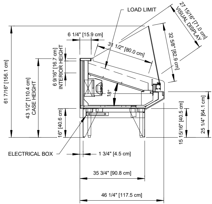
43" PROFILE
