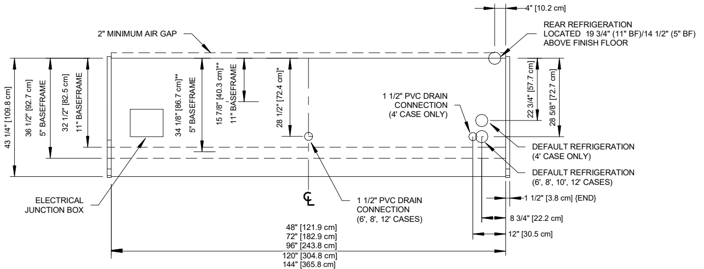
11" BASEFRAME
