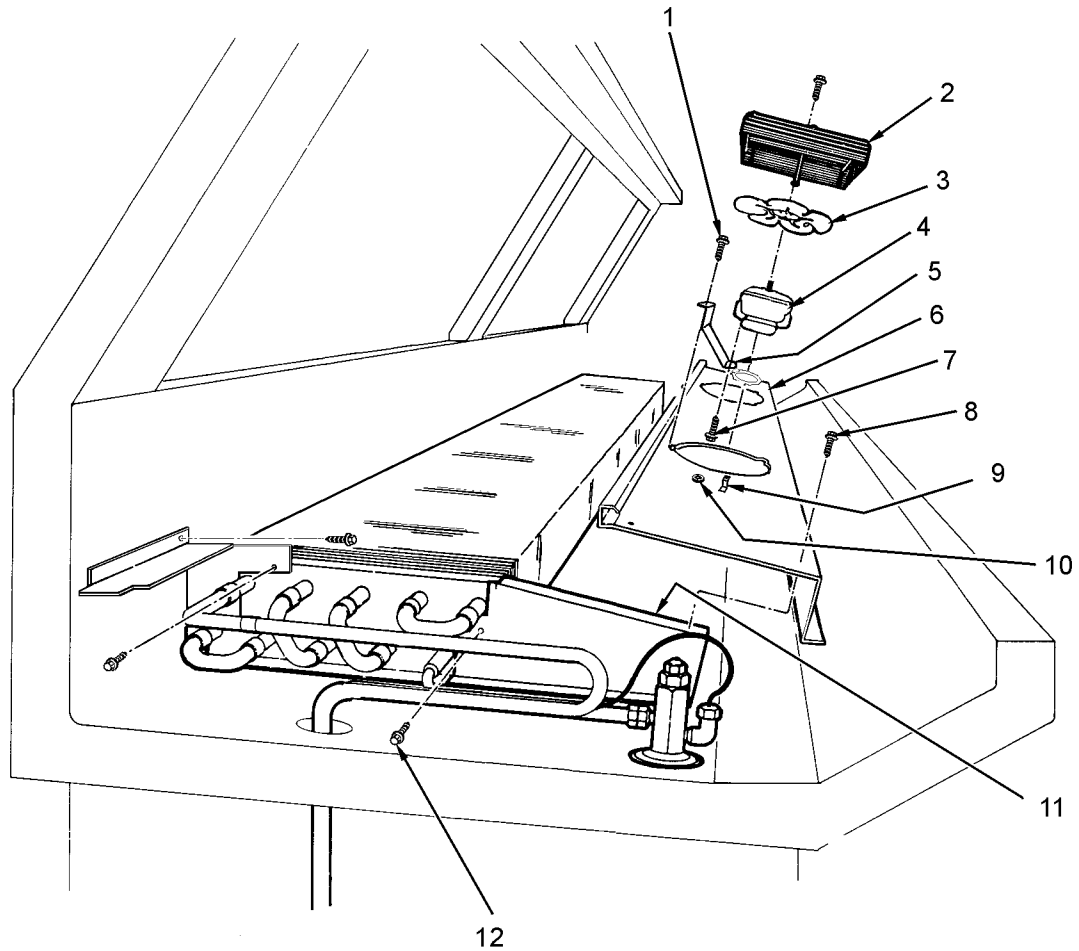
6', 8' and 12' Merchandiser
