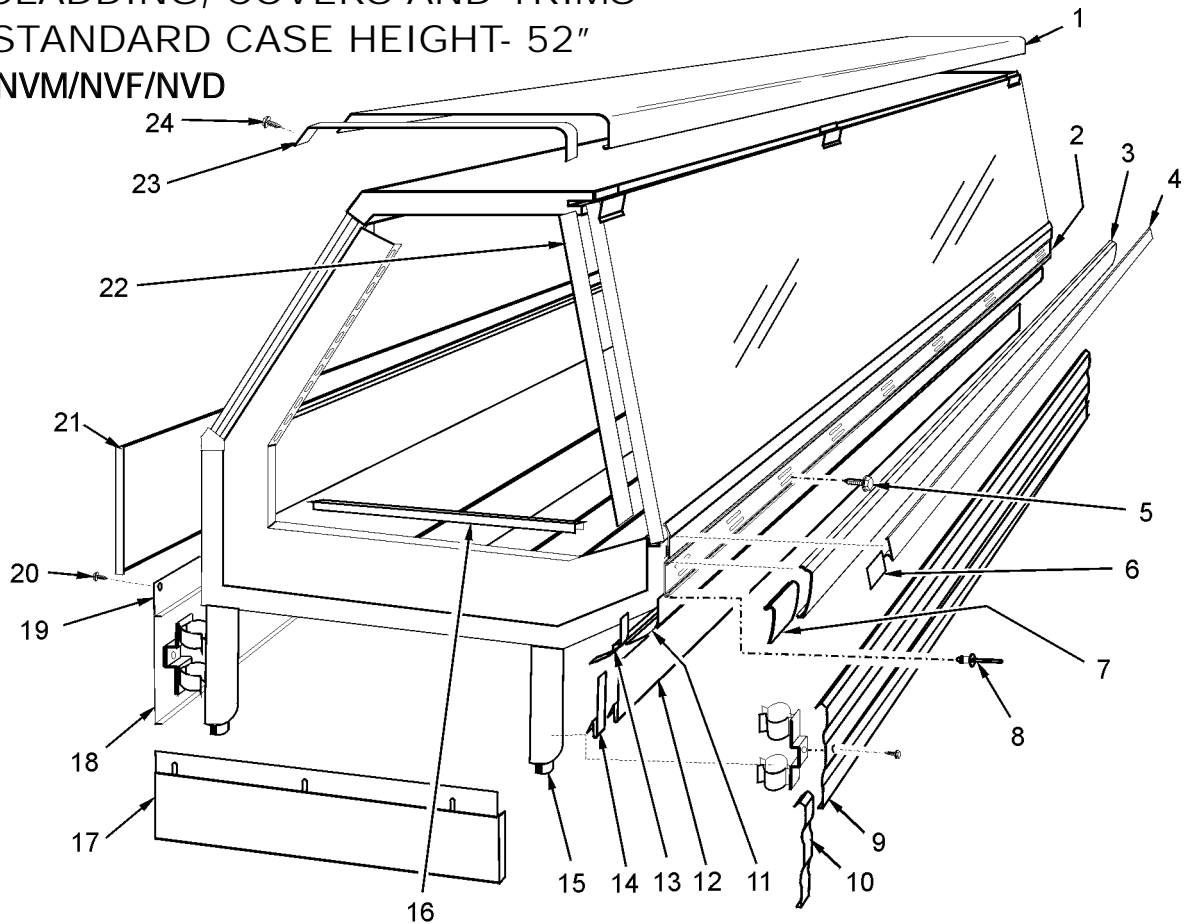
6', 8' and 12' Merchandiser
