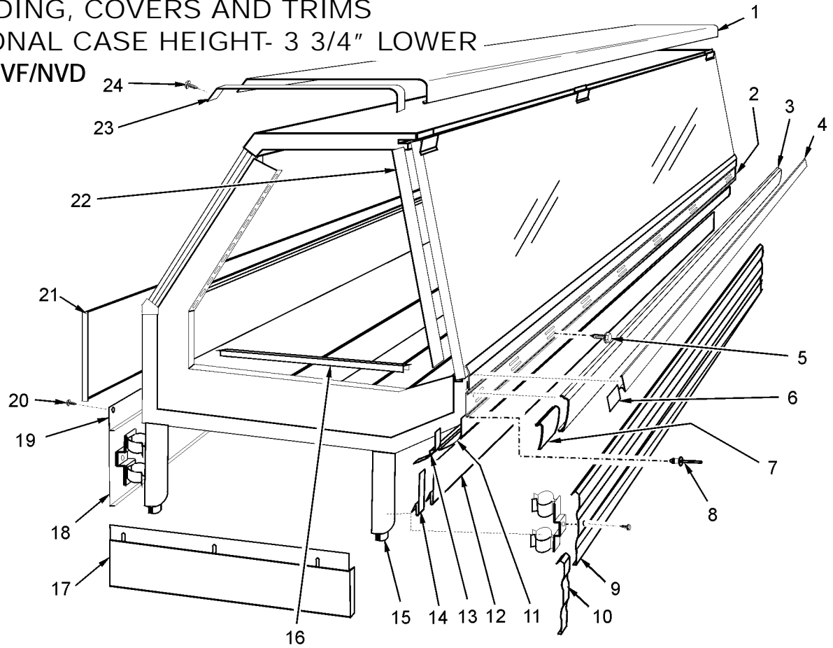
6', 8' and 12' Merchandiser
