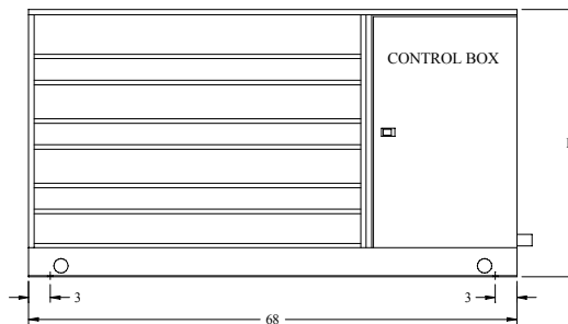
FRONT VIEW - 2 FAN MODEL DC/DL/DS
