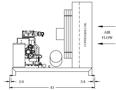
RIGHT SIDE VIEW MODEL DE
