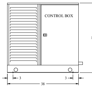
FRONT VIEW - 1 FAN MODEL DC/DL/DS
