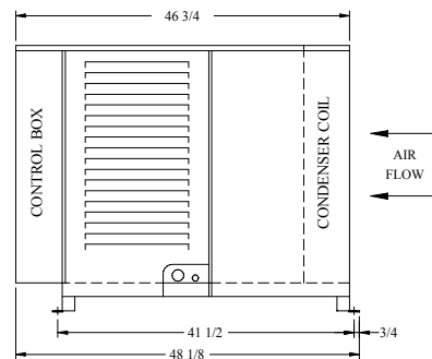
RIGHT SIDE VIEW MODEL DC/DL/DS
