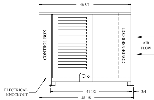
RIGHT SIDE VIEW MODEL DC/DL/DS
