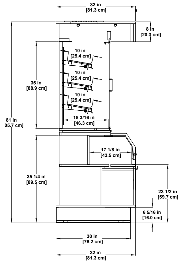
BWU-RB | Dry Multi-deck Display
