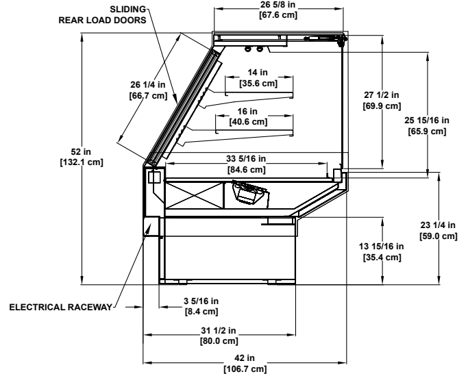
SMD-R | Refrigerated/Vertical Glass Multi-deck Display
