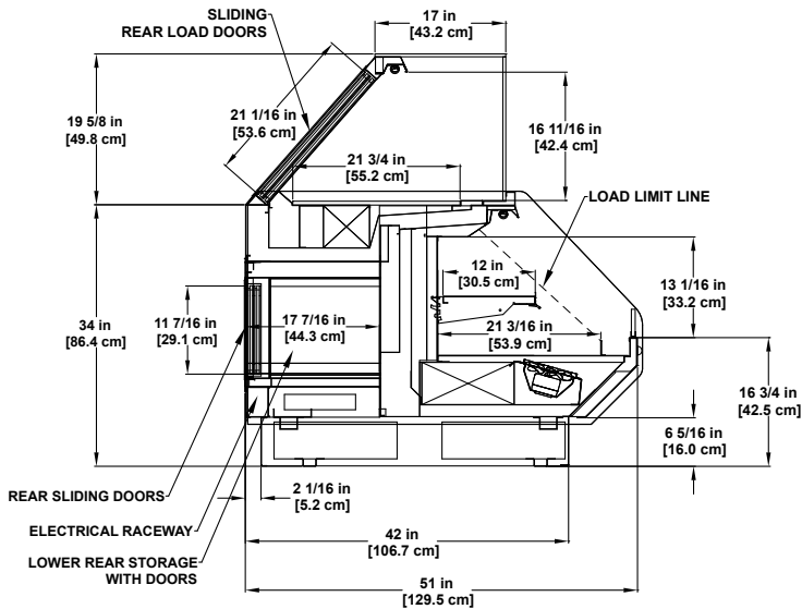
PTD-GSD-R Refrigerated Service Dome and Self-service Base
