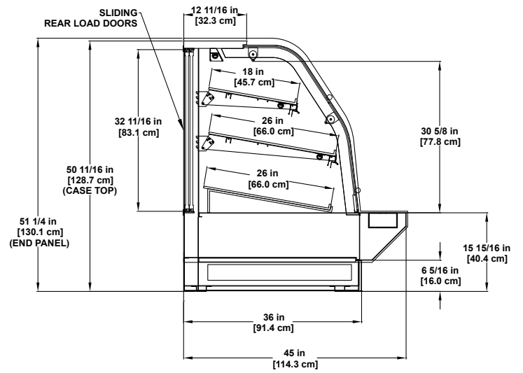
BLF-RB | Dry Multi-Deck Display
