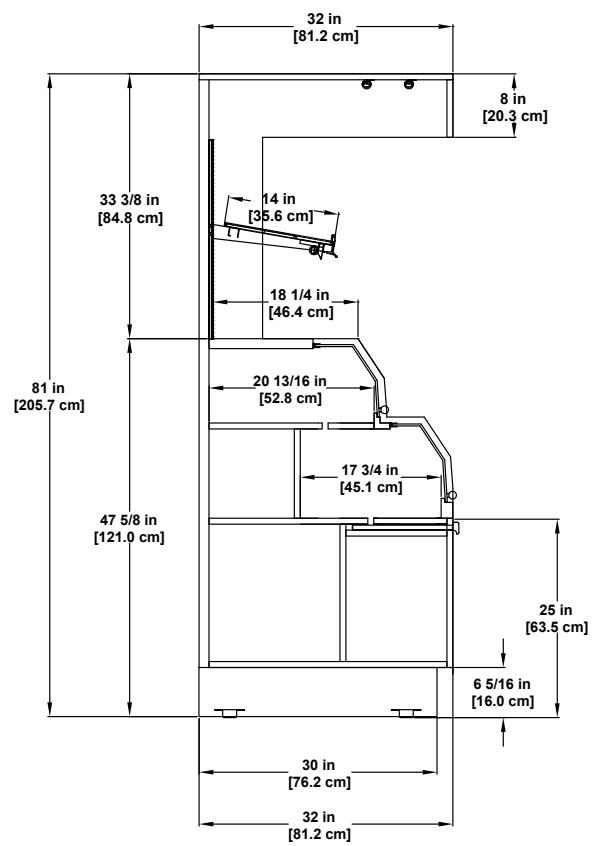
BWS-RB | Dry Multi-deck Display
