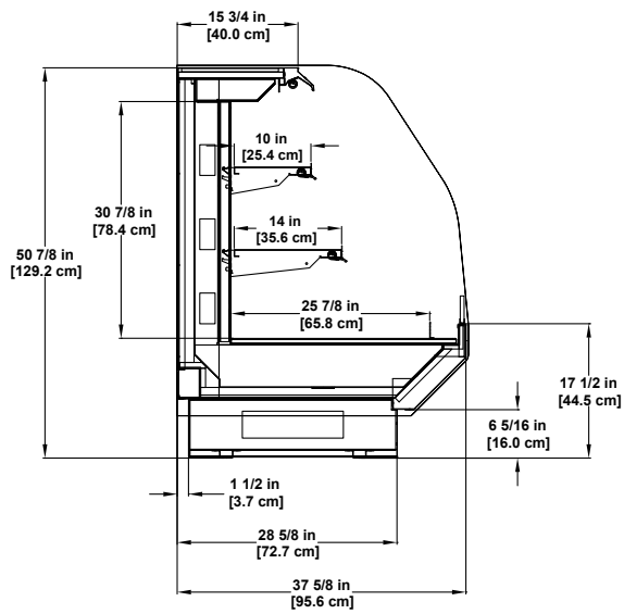
BLF-SD | Dry Multi-deck Display
