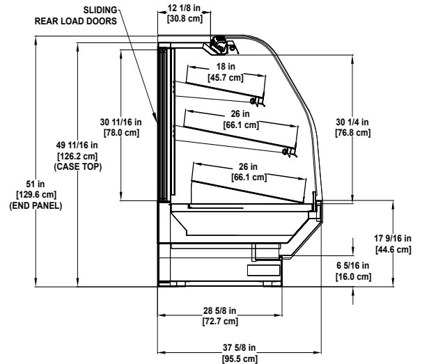
BLF-D | Dry Multi-deck Display
