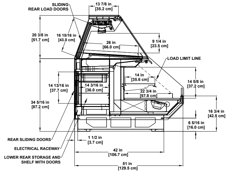
PTD-RGC M S Coolgenix Dome Refrigerated Base
