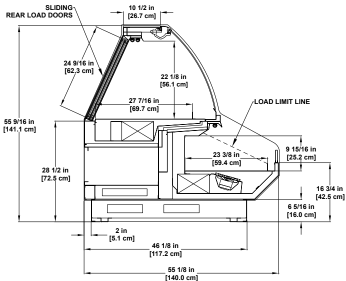
SD-R Spherical B B D Refrigerated Dome & Base
