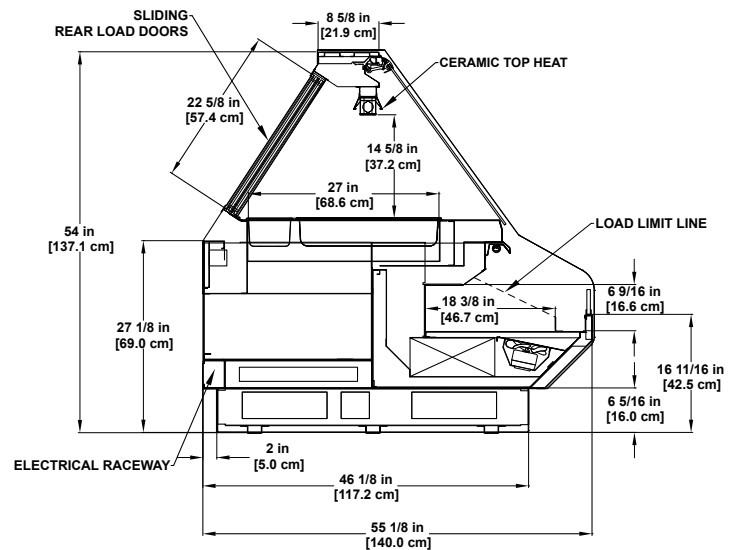
SDH-H D Hot Dome Refrigerated Base
