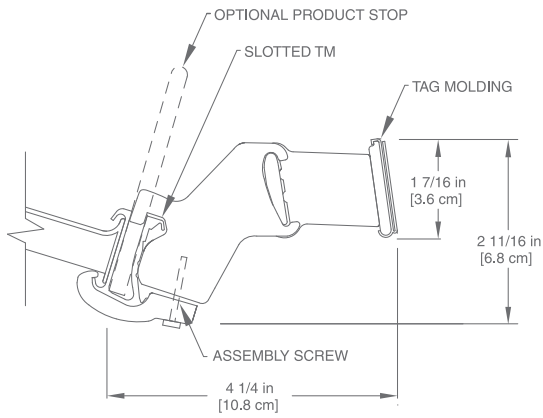
ANGLED SHELF APPLICATION
