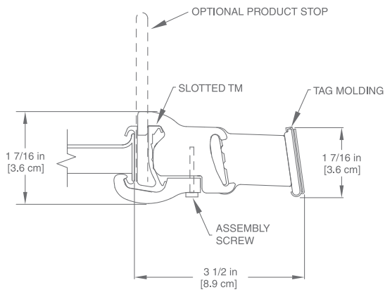
FLAT SHELF SLOTTED APPLICATION
