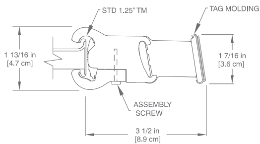
FLAT SHELF STANDARD APPLICATION
