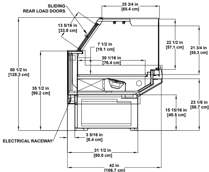
GSD-R | Refrigerated Single-deck Display
