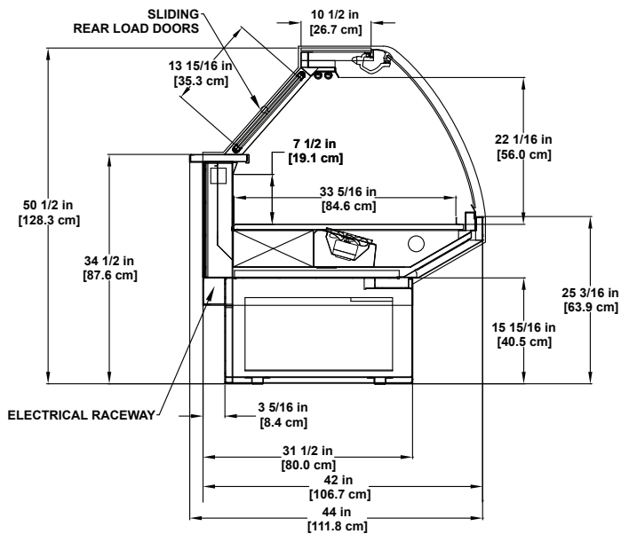
SSD-R | Refrigerated Single-deck Display
