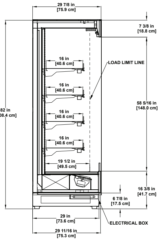
QC-R Refrigerated Multi-deck Display
