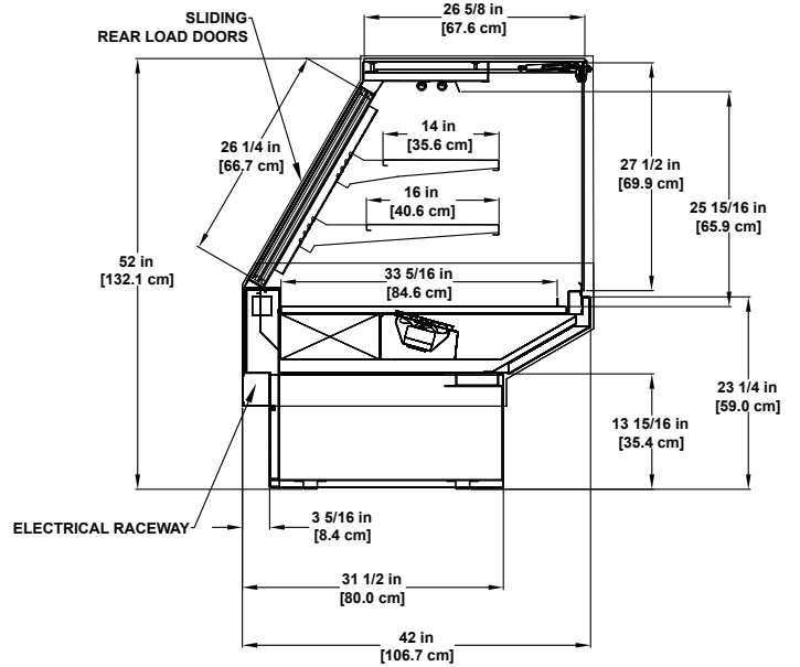
SMD-R | Refrigerated / Vertical Glass Multi-deck Display
