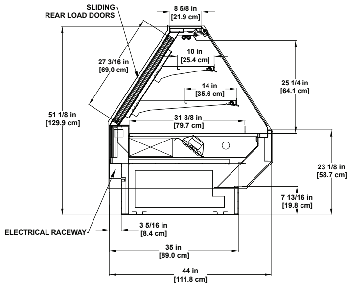
BMD-R | Refrigerated Multi-deck Display
