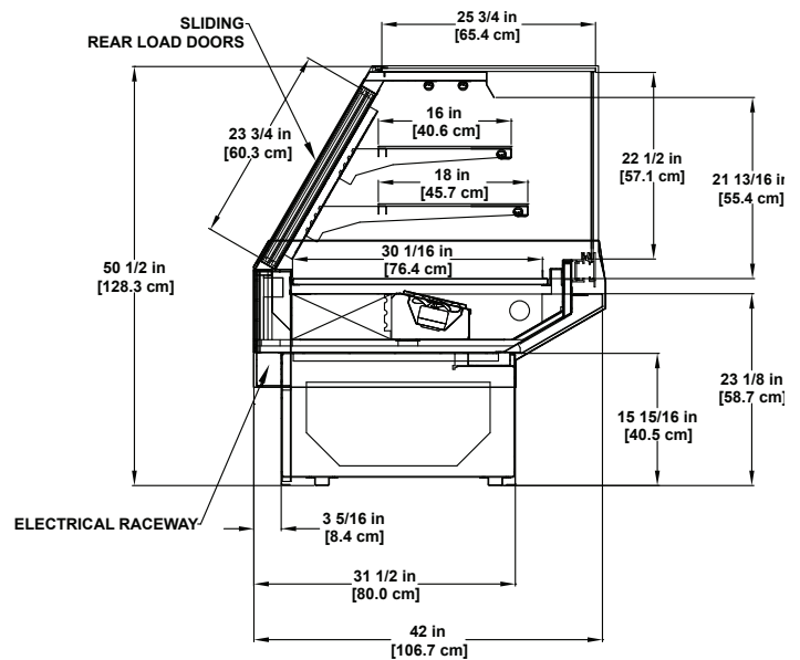
GMD-R | Refrigerated Multi-deck Display
