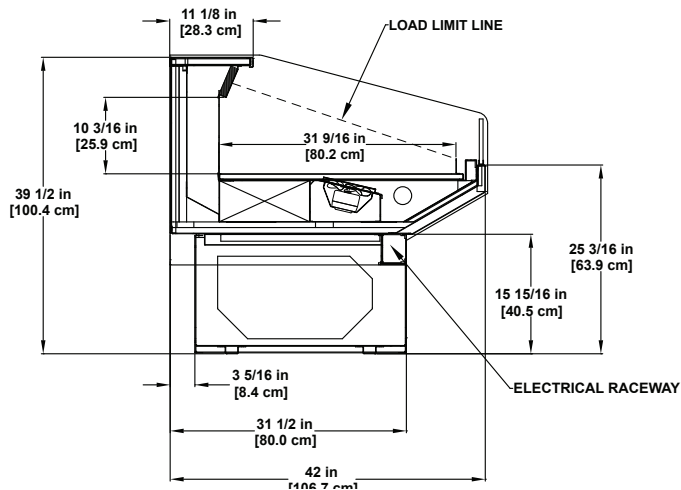
DLPC-R Refrigerated Single-deck Display
