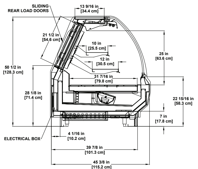
SSA-R | Refrigerated Multi-deck Display
