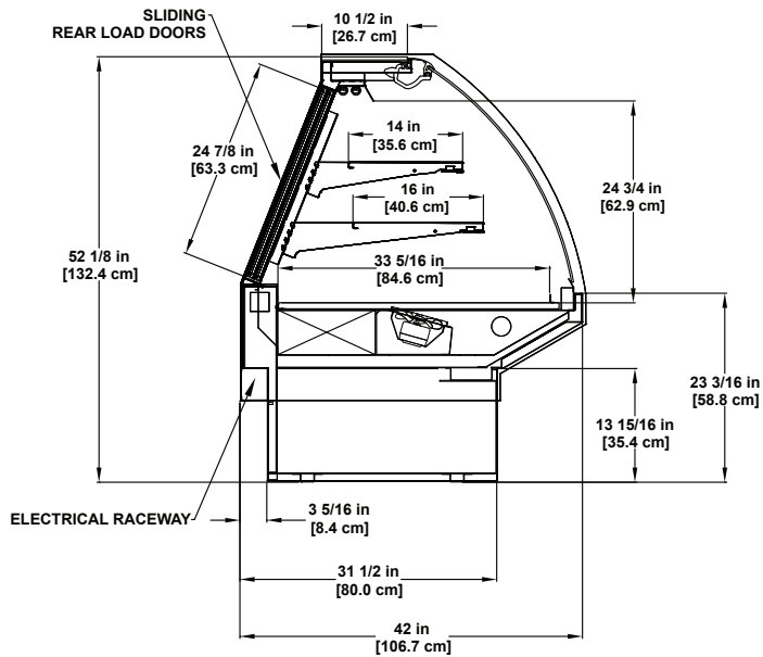
SMD-R | Refrigerated Multi-deck Display
