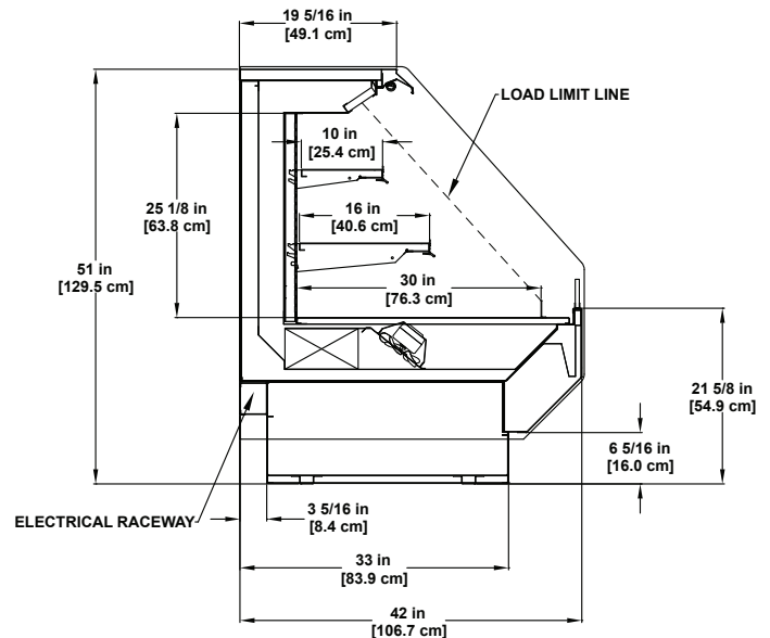
PF-R Refrigerated Multi-deck Display
