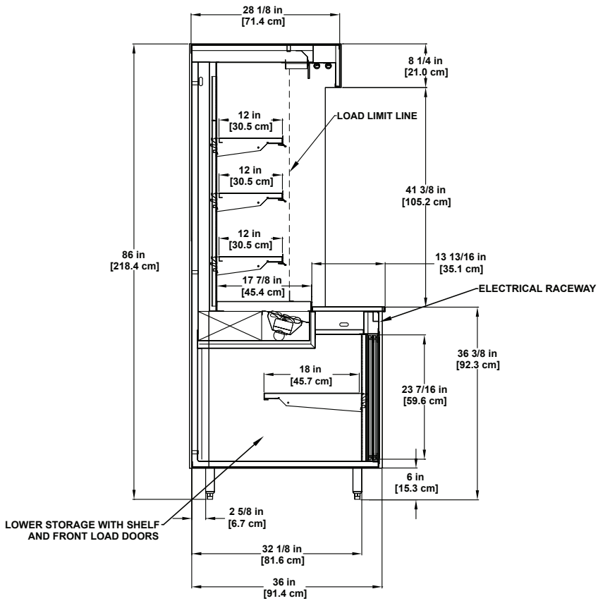
DB-R Refrigerated Multi-deck Display
