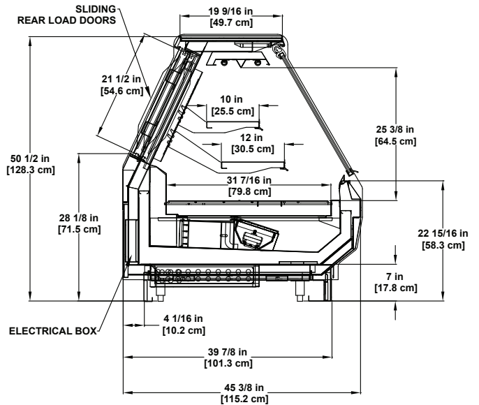
SSF-R | Refrigerated Multi-deck Display
