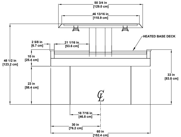
DI-H Hot Single-deck Display
