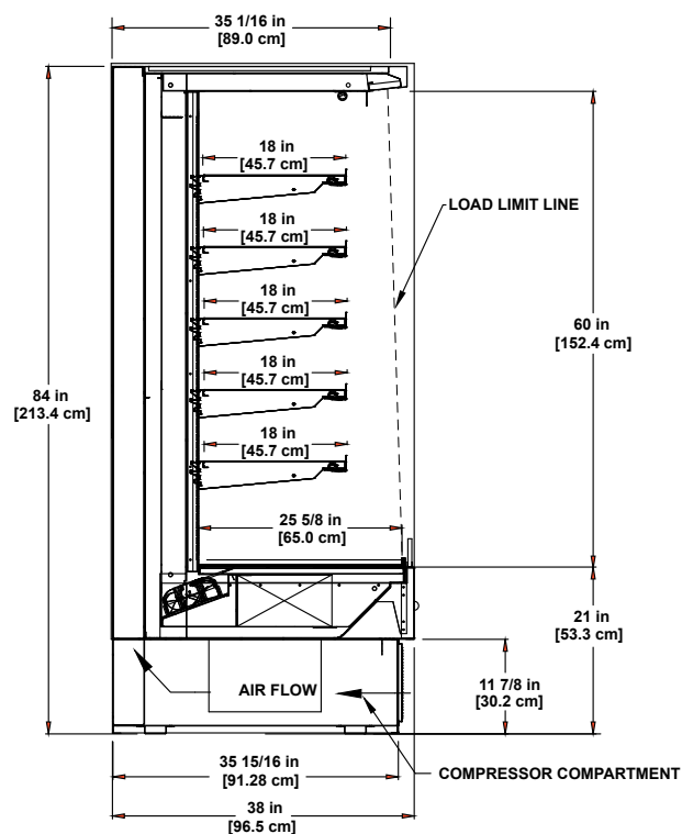
PF-SC-84 | Refrigerated Multi-deck Display
