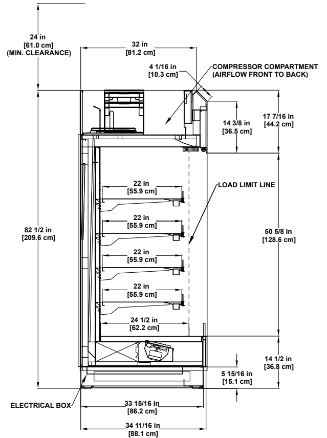
QTM Refrigerated Multi-deck Display
