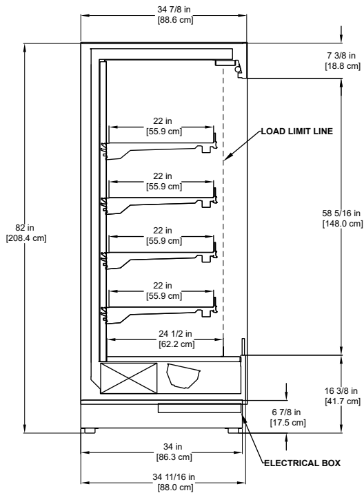
QC-R Refrigerated Multi-deck Display
