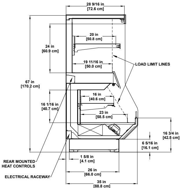
HTPT Refrigerated / Hot Multi-deck Display
