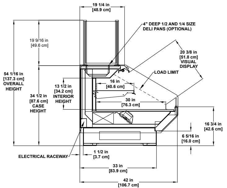
PT-R | Refrigerated Multi-deck Display Available with Refrigerated Rear Storage
