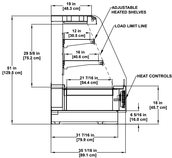
PFH Hot Multi-deck Display Conduction Heat
