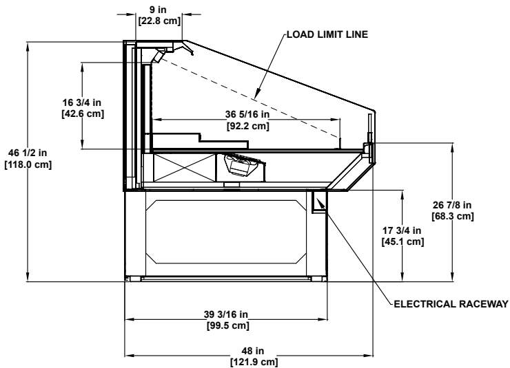
HSC-R Refrigerated HSC-SC Single-deck Display
