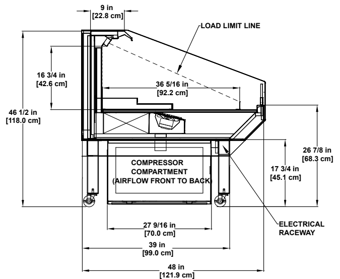
HSO-SC Refrigerated Single-deck Display
