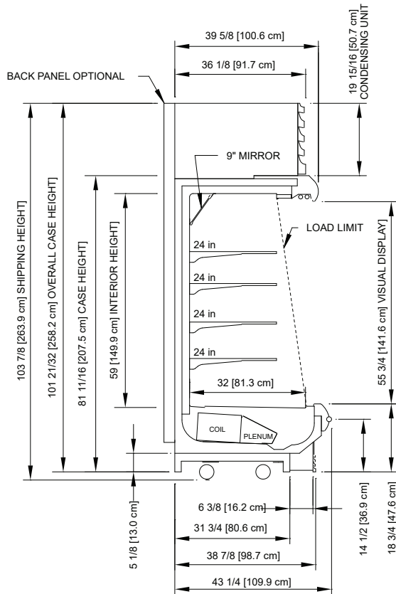
O5DMA-NRG Refrigerated 4', 6', 8' & 12' Multi-deck Display
