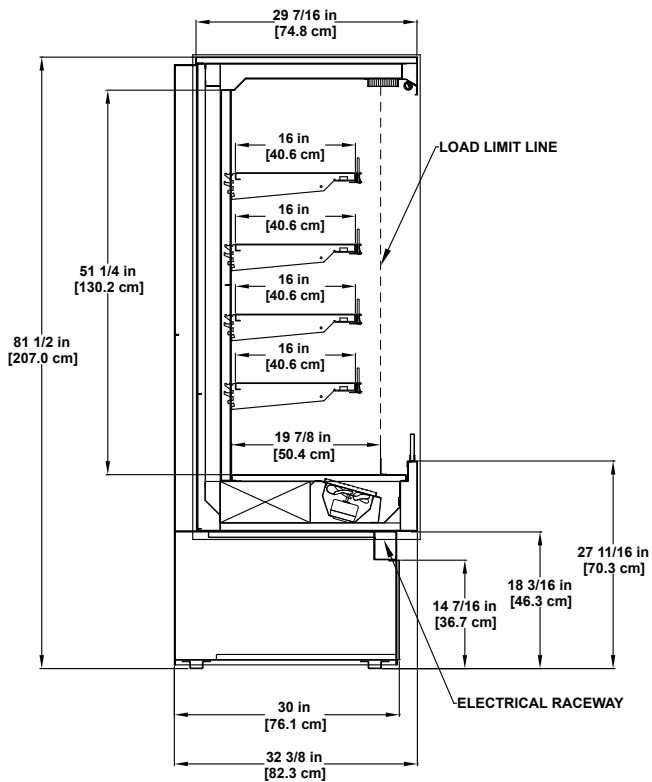
CF-S-SC | Refrigerated 4' Multi-deck Display
