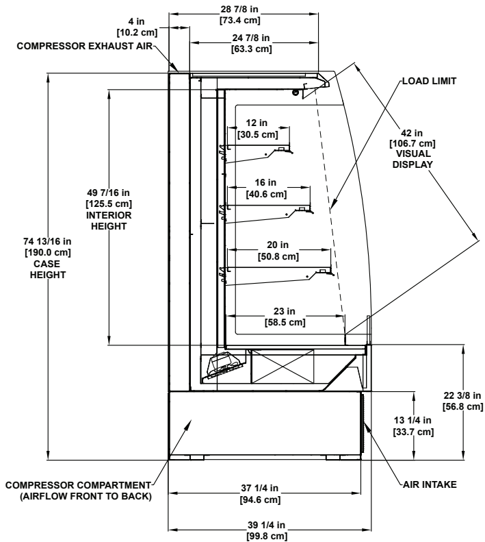
PF-S-K Refrigerated 4' Multi-deck Display
