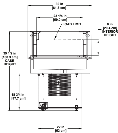
MIDA | Refrigerated 3'X3' Single-deck Display
