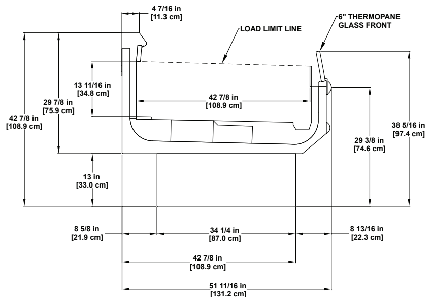
OWMA | Refrigerated 8' Multi-deck Display
