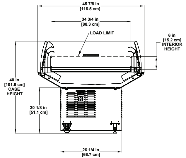
MIDA | Refrigerated 4'X4' & 4'X8' Single-deck Display
