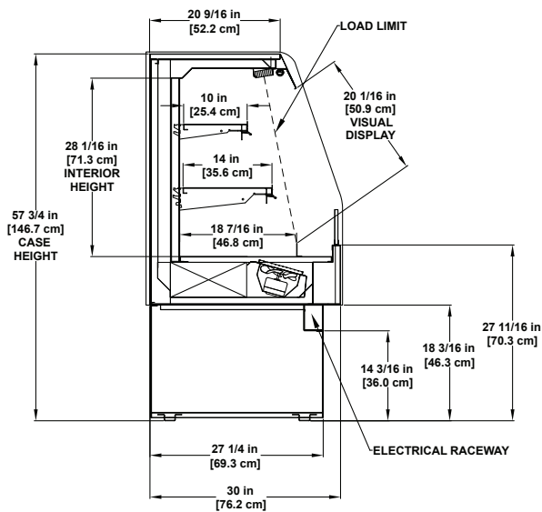
CF-SC | Refrigerated 4' & 6' Multi-deck Display
