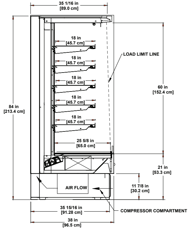
PF-SC-84 Refrigerated 4' Multi-deck Display
