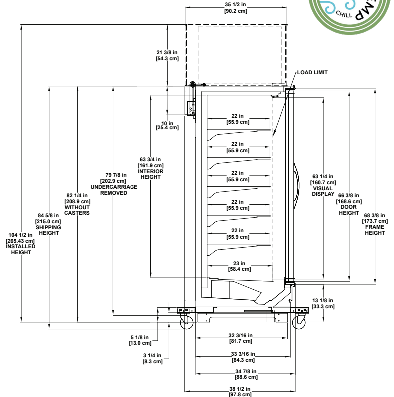
JNRBHS-A-NRG Refrigerated 1, 2, 3, 4, 5 Doors Reach-In Display
