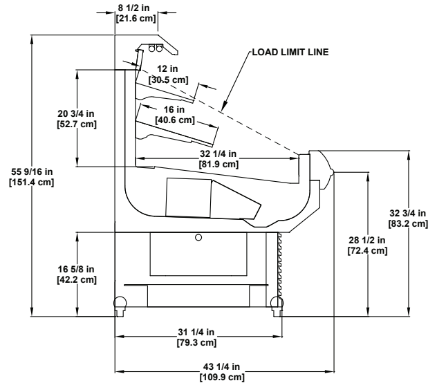
02.5UMA-NRG | Refrigerated 4', 6', & 8' Multi-deck Display
