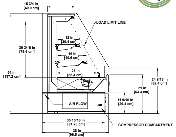
PF-SC-54 Refrigerated 4' Multi-deck Display
