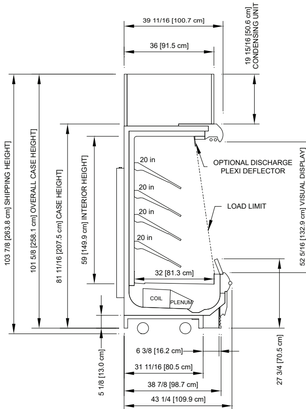
O5MA-NRG Refrigerated 4', 6', 8' & 12' Multi-deck Display
