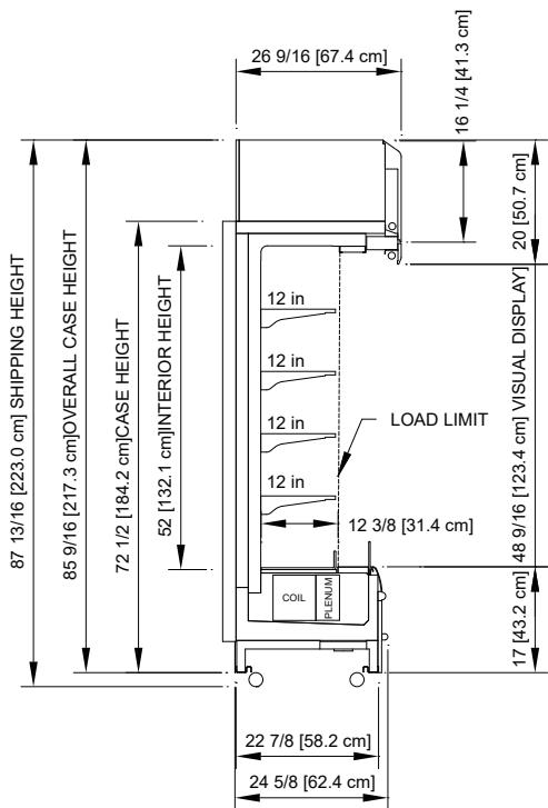
ONNSA Refrigerated 39" & 47" Multi-deck Display
