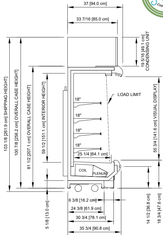
ON5DMXA-NRG Refrigerated 6' & 8' Multi-deck Display
