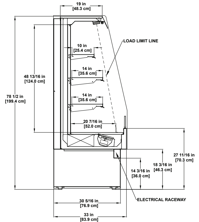
CF-FS-SC | Refrigerated 6' Multi-deck Display
