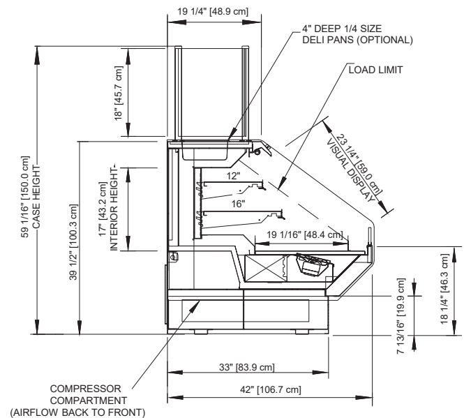
PT-SC | Refrigerated 4' & 6' Multi-deck Display
