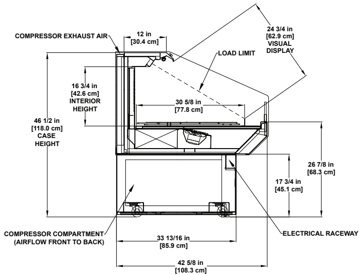
HSC-S-K Refrigerated 2', 3' & 4' Single-deck Display Closed Base
