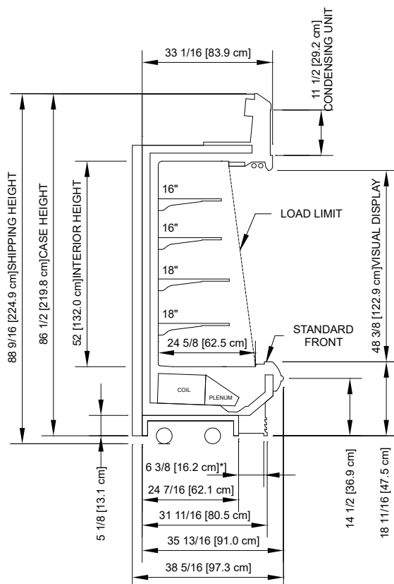
ONUA Refrigerated 44-1/2", 4' & 6' Multi-deck Display
